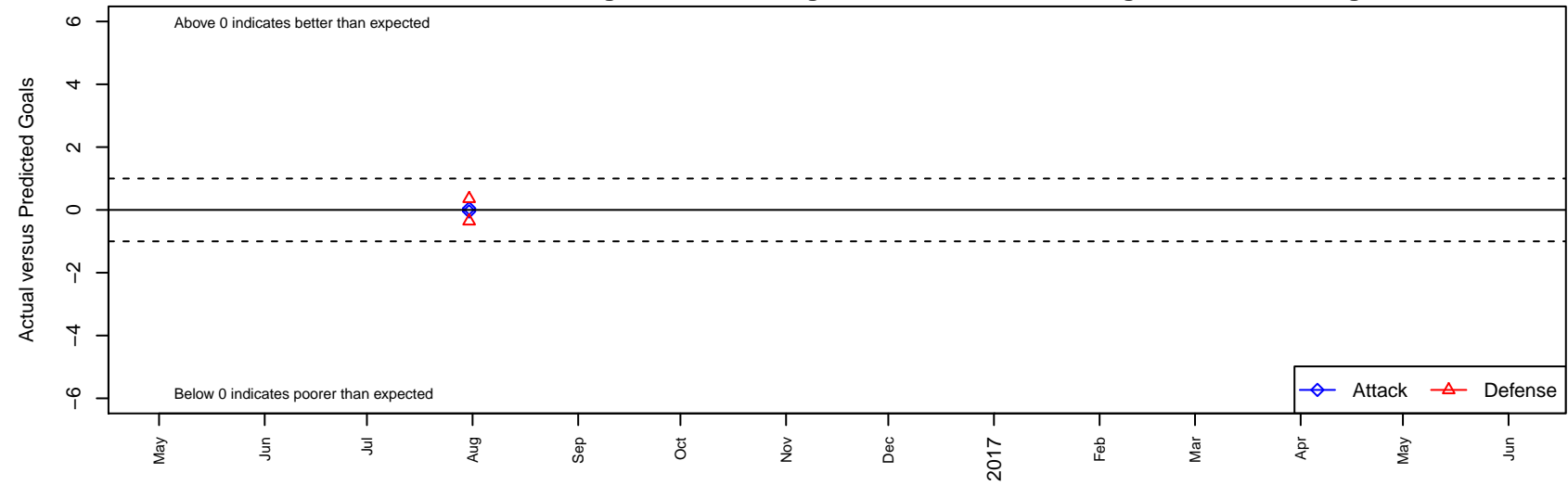
Avalanche FC Apex Black B99 Dots are actual minus expected GF (blue circles) and GA (red triangles). Blue line is smoothed change in attack strength. Red is smoothed change in defense strength.
